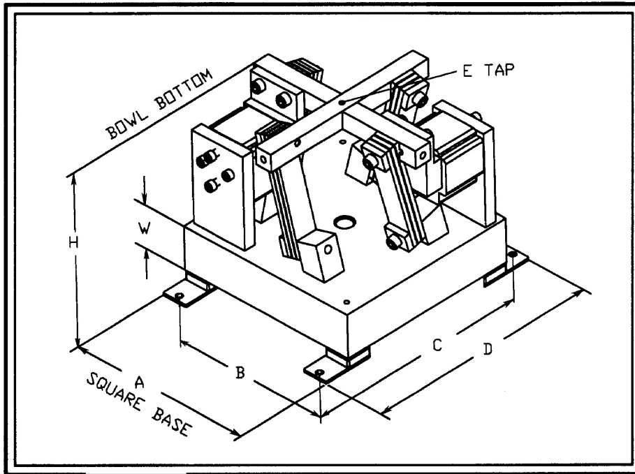
24" CCW BOWL DRIVE BASE (4) POSTS - (2) COILS
