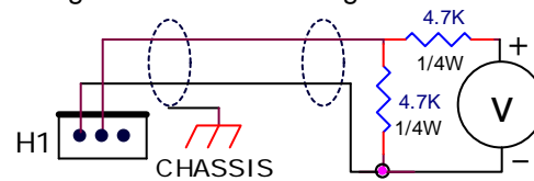
0-10VDC Input Diagram
