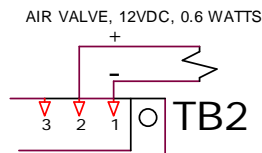
Typical relay or air valve wiring
